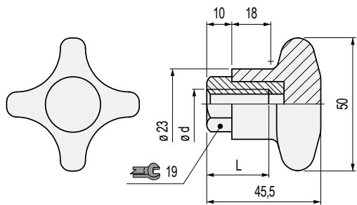
Tightening knob
