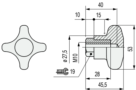
Tightening knob
